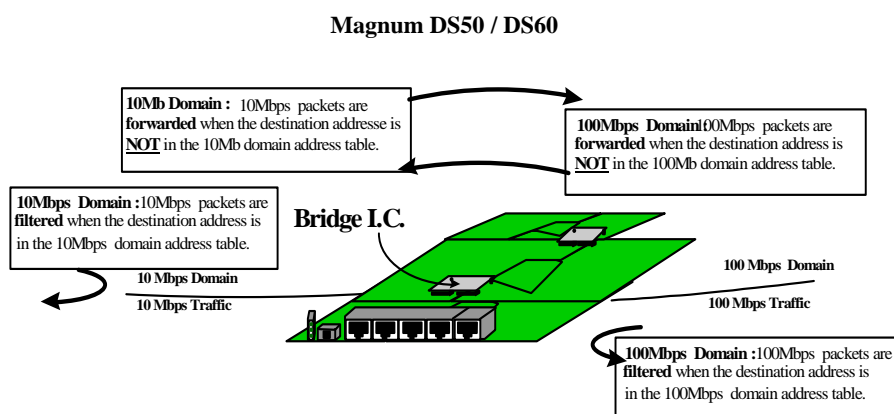
Figure 4.1 : Filtering and Forwarding at port (1-5) in DS50 / DS60 Dual-speed Hubs
